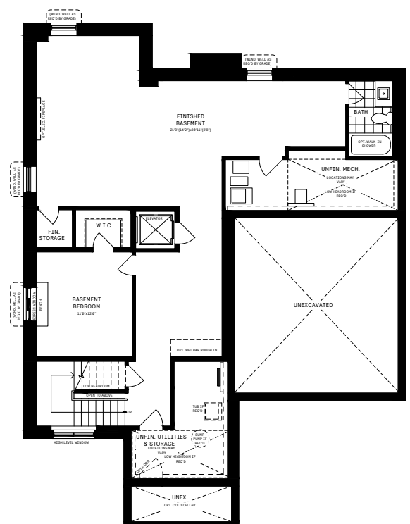
10 Finished Basement Package
