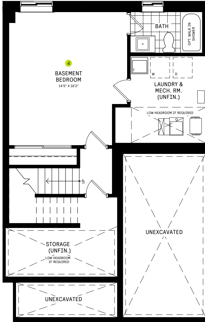
4 Larger Basement Bedroom
